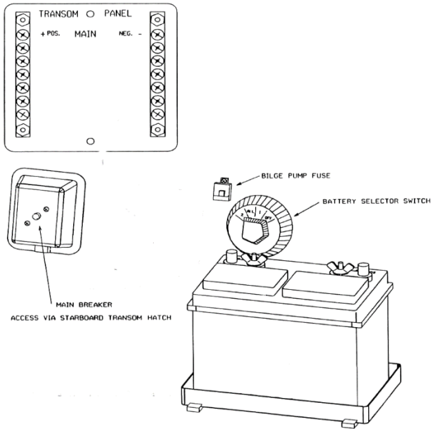
Transom Panel (showing a battery switch)
