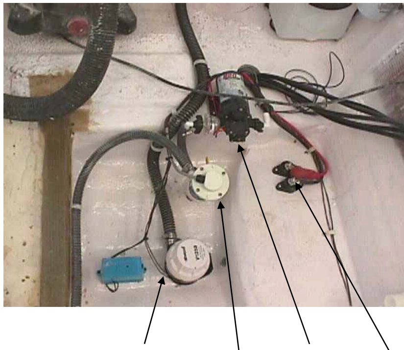
Bilge pump, baitwell pump, washdown pump, engine posts
