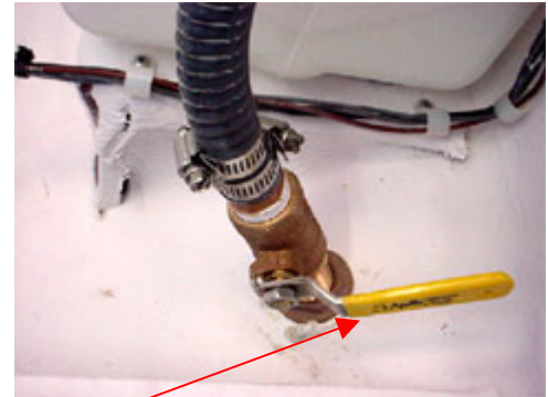
Seacock lever is shown in the closed position.
