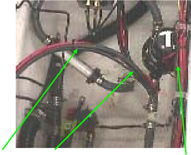
Raw Water Filter, Seacock (shown in open position), On-demand Pump Bilge Layout
