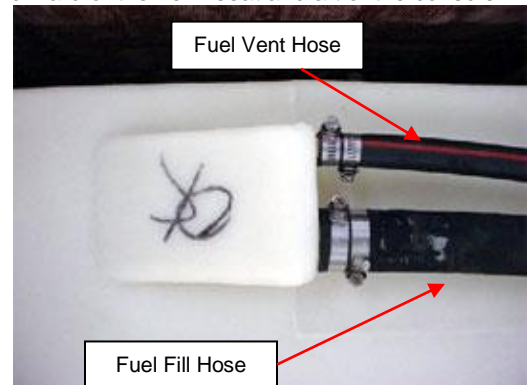
Located below the access pie installed forward of the helm seat and aft of the console.
