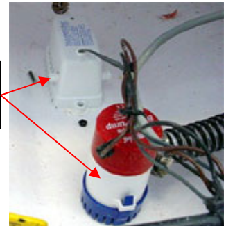
Bilge pump & float switch
