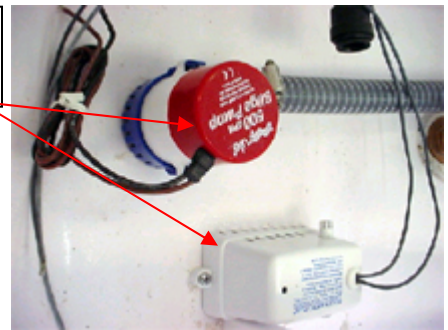
Forward bilge pump with float switch
