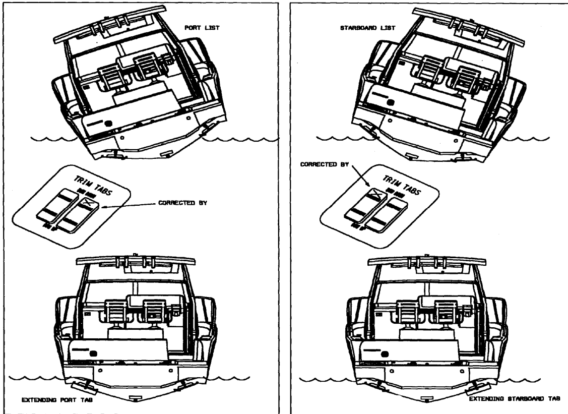
Trim Tabs and Pump Location (pump location may vary)
