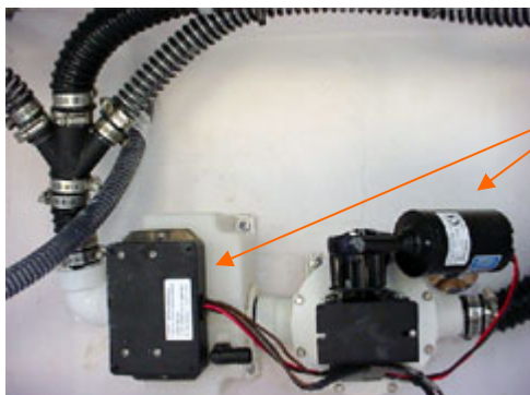
Forward Fish Box Pump and Collector Box
