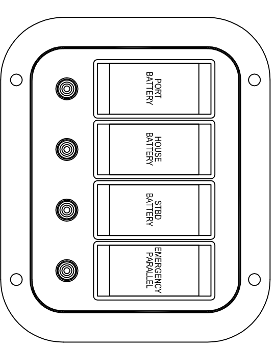
FACE VIEW
